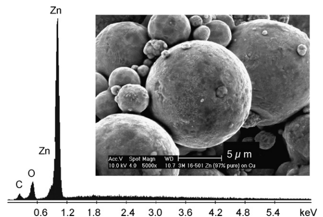
Fig. 6. Detail SEM picture of Zn anode particles and corresponding XEDS spectrum for IOS-C-1.
