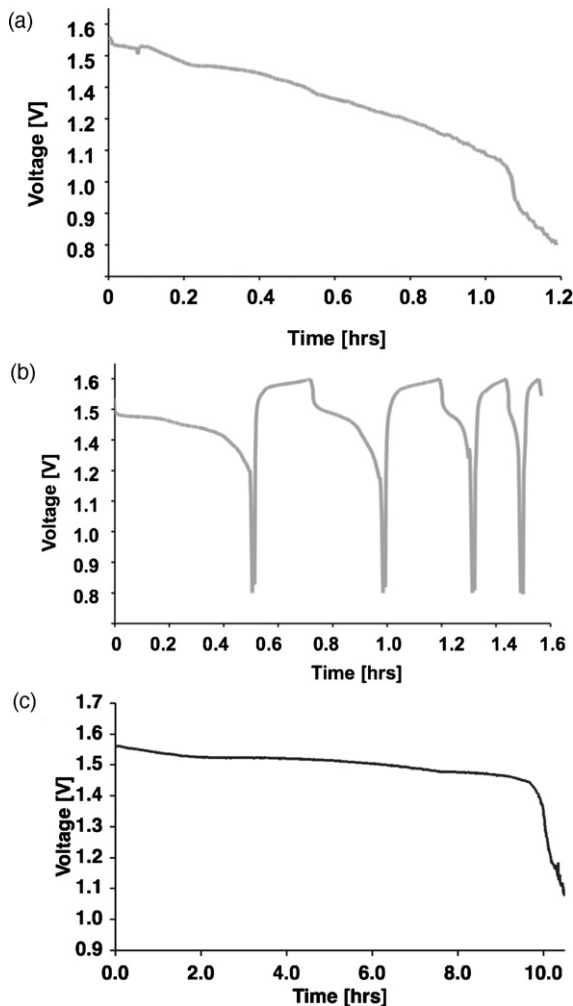
Fig. 9. Discharge profiles for O(mm 2 ) batteries: (a) IOS-M-1 1st cycle 2.5 μA (~0.7 C), (b) IOS-M-1 2.5 μA (~0.7 C), and (c) IOS-M-2 25 nA (~C/150).
