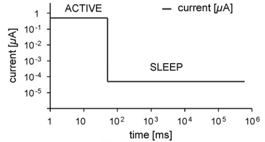
Fig. 2. WIMS-ERC IOS microchip duty cycle.
