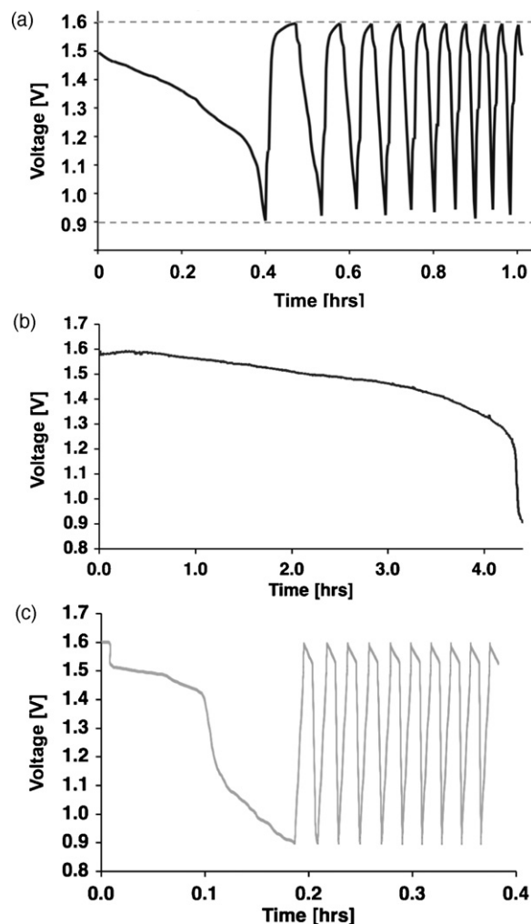
Fig. 8. Discharge profiles for O(cm 2 ) batteries: (a) IOS-C-1 250 μA (~1.4 C), (b) IOS-C-2 2.5 μA (~C/70), (c) IOS-C-3 250 μA (~1.4 C).
