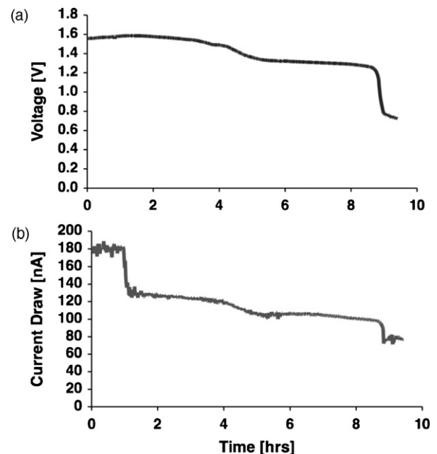
Fig. 10. Discharge profile for on-chip battery: (a) IOS-X-1 discharge voltage and (b) IOS-X-1 discharge current (~100–200 nA).
