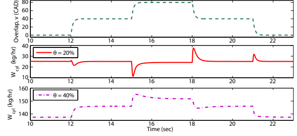
Fig. 6. Cylinder air charge rate W_{cyl} response of the turbocharged engine on VVT overlap v step changes; engine speed is 2000 RPM and throttle is fixed at \theta = 20\% (second plot) and \theta = 40\% (third plot).
