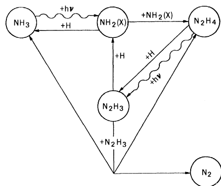
Fig. 1. Schematic of ammonia photochemistry.
