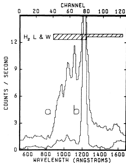
Fig. 5 (left). Airglow spectra from Jupiter. A portion of the northern auroral zone lay within the slit for spectrum a. Spectrum b was recorded near the equator and contains no radiation from the sharply localized auroral zones at high latitudes. The zero for spectrum a is shifted upward by 1 count per second. Noise and scattering within the instrument have been removed from these spectra. Both spectra include emission in the Lyman and Werner bands of H 2 in the indicated wavelength regions as well as H Ly \alpha . The equatorial brightness in the Lyman and Werner bands is about 5.5 kR. An additional feature not due to H or H 2 emission is present in slightly different forms near 1570 Å in both spectra. The origin of this radiation is unknown. Fig. 6 (right). Occultation of \alpha Leo (Regulus) by Jupiter. The stellar light recorded in two wavelength intervals is represented as a function of relative altitude. Gradual absorption at 976 to 1078 Å is attributed to H 2 , whereas the abrupt onset of absorption at 1273 to 1375 Å is attributed to hydrocarbons. The residual signal after the hydrocarbon occultation is a combination of high-energy particle background and Jupiter's dayglow.
