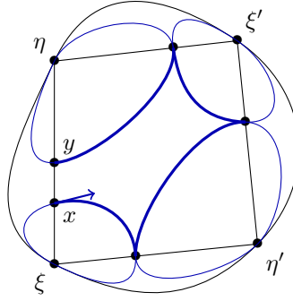
Figure 5: Illustration of computations (6.9), where d_{\Omega}(x, y) = B(\xi, \xi', \eta, \eta')
