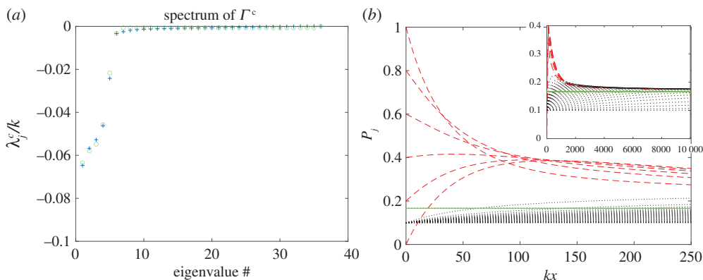
Figure 5. Results for the Gaussian covariance with \ell = 1/k . (a) The eigenvalues \lambda_j^c of \Gamma^c are shown with blue crosses and the estimates \lambda_j^c = \theta_{N+1-j} with \theta_j given by (6.3) are shown with the green circles. (b) Evolution of the mode powers with increasing range x . The surface mode powers are shown with red dashed lines, the body mode powers are shown with black dotted lines, and the solid green line is the average mode power. The inset corresponds to longer propagation distances ( kx up to 10^4 ) and displays the evolution toward equipartition, albeit very slowly for the body modes. (Online version in colour.)
