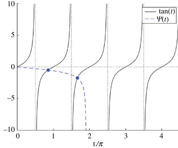
Figure 6. Determination of the solutions of the equation \psi(t) = \tan(t) with kd\sqrt{n^2 - 1} = 6 . Here there are N_s = 2 solutions (the blue dots). (Online version in colour.)
