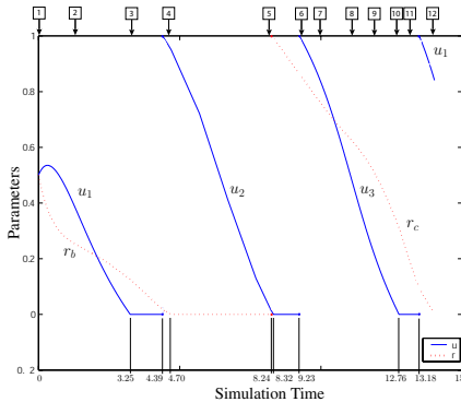
Figure 11. The trajectory and sequence of parameters u_1, u_2, u_3 on curves C_1, C_2, C_3 and r_a, r_b, r_c on curves C_a, C_b, C_c for the simulation shown in Figure 10. Transition times are indicated.
