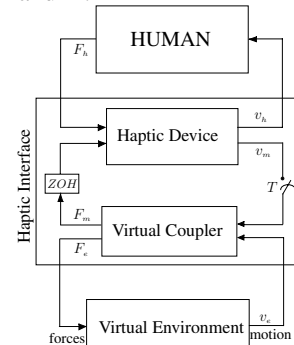
Figure 2. Block diagram of haptic rendering.
