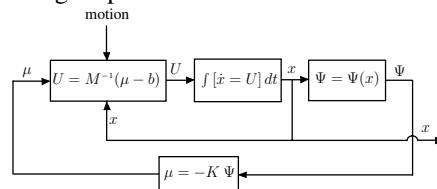
Figure 5. Block diagram of the alternative implementation
