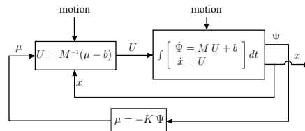
Figure 4. Block diagram showing inner feedback linearization loop and outer linear control loop
