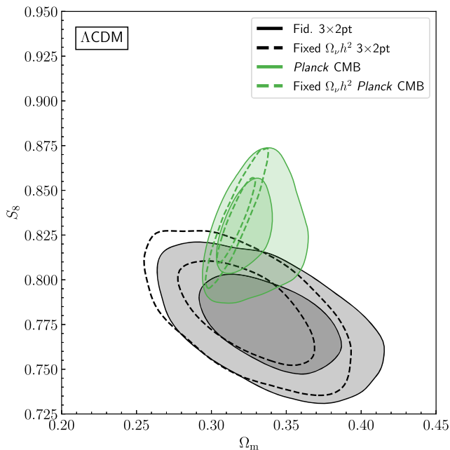
FIG. 28. A comparison of the fiducial 3 \times 2 pt analysis (black solid) with one that fixes the neutrino mass density to fixed minimum value (black dashed). We make a similar comparison for the Planck CMB data (green solid and dashed).
