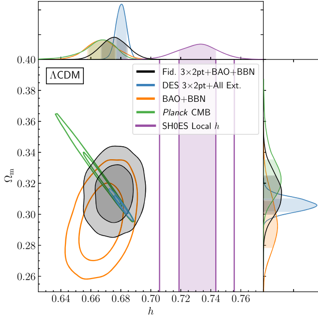
FIG. 20. Marginalized constraints on h and \Omega_m in the \Lambda CDM model are compared to the SH0ES local determination of h . Planck CMB data and the combination of BAO and BBN provide comparable uncertainties on h compared to the local constraint. Adding DES 3 \times 2 pt to BAO and BBN improves the constraint on h slightly due to 3 \times 2 pt providing additional information on \Omega_m , while the combination of DES 3 \times 2 pt and all nonlocal external data provide a constraint on h that is a factor of 3–4 more powerful than the local determination.
