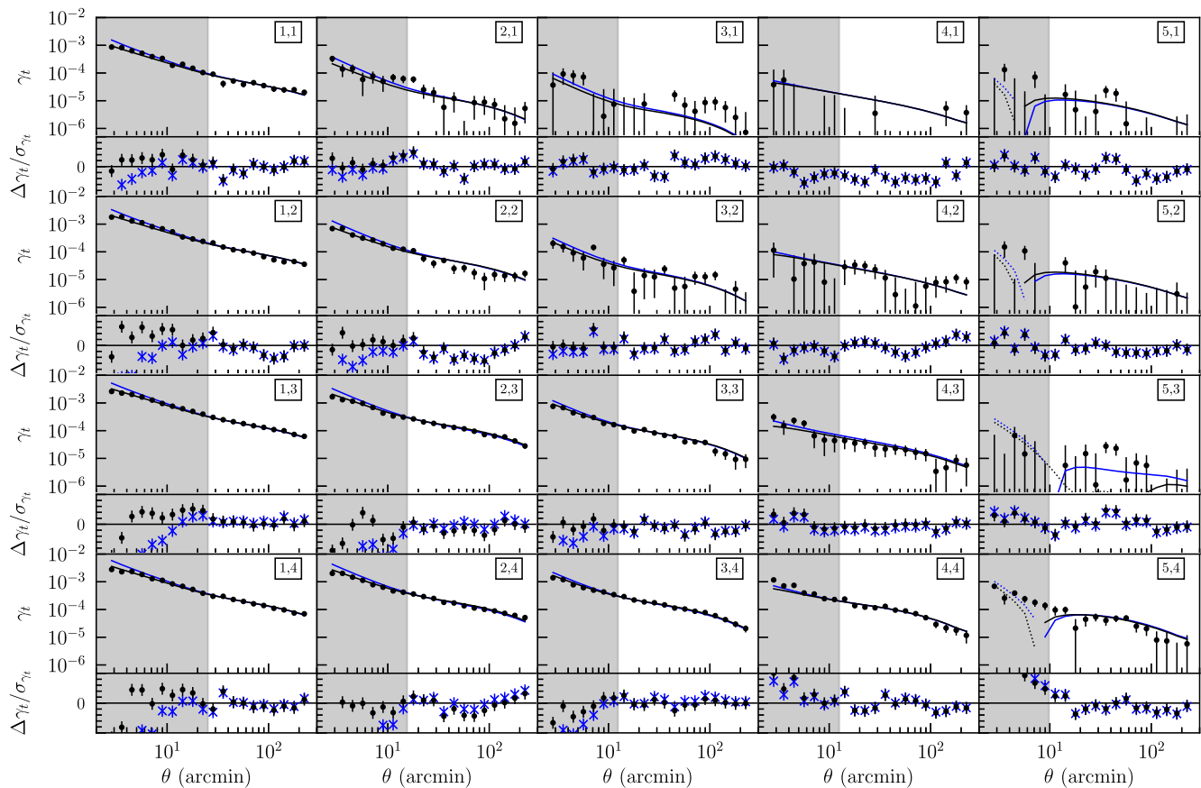
FIG. 23. The measured \gamma_t(\theta) correlation functions for each tomographic bin combination using the redMaGiC sample, with labels as described in Fig. 3. The best-fit \Lambda CDM model from the analysis with fixed X_{\text{lens}} is plotted as the solid line in the top part of each panel, with dotted curves indicating a negative model fit. The best-fit model marginalizing over X_{\text{lens}} is shown in blue. The bottom part of each panel shows the fractional differences between the measurements and the model prediction, (\gamma_t^{\text{obs}} - \gamma_t^{\text{th}})/\sigma_{\gamma_t} (with y-axis range \pm 5\sigma ). In both panels, 1\sigma error bars are included. Angular scales not used in the cosmological analysis are indicated by grey shading, which are excluded on small scales where the linear galaxy bias assumption breaks down.
