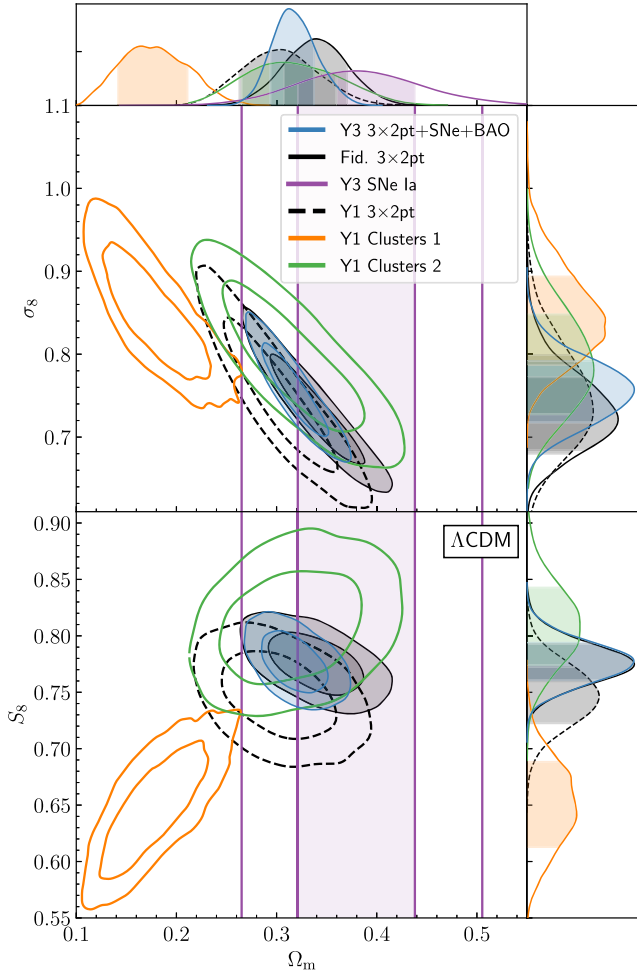
FIG. 13. A comparison of the marginalized constraints on parameters in the \Lambda CDM model from a variety of DES probes: large-scale structure and weak lensing ( 3 \times 2 pt; Y3—black solid, Y1 reanalyzed—black dashed), type Ia supernovae (purple), galaxy cluster number counts and masses (orange and green), and BAO. The combination of DES Y3 3 \times 2 pt, SNe Ia, and BAO is shown in blue. Going from Y1 to Y3, we find approximately a factor of two improvement in the 3 \times 2 pt constraint in \Omega_m - S_8 plane.
