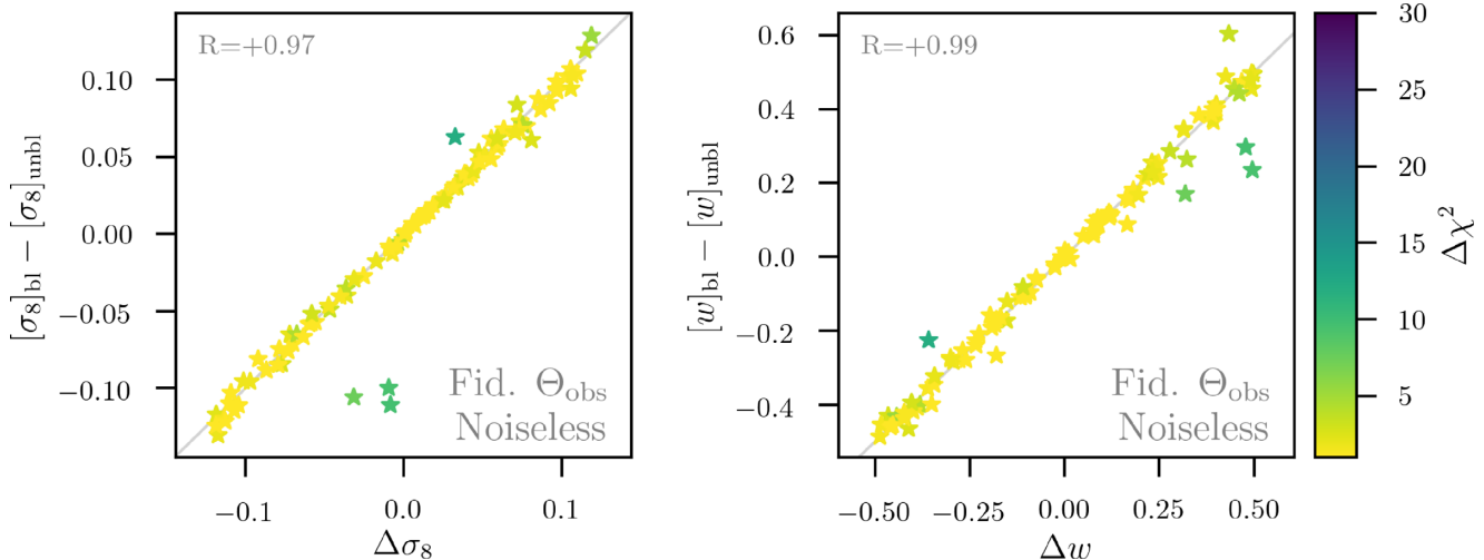
Figure 7. Relationship between the input blinding shifts (horizontal axes) in \sigma_8 (left-hand panel) and w (right-hand panel) and the output shifts in best-fitting values of those same parameters. The colour scale shows \Delta\chi^2 and the diagonal grey line shows the case where the output shifts are exactly equal to the input shifts. Both plots show data from the same 100 realizations for noiseless simulated data.
