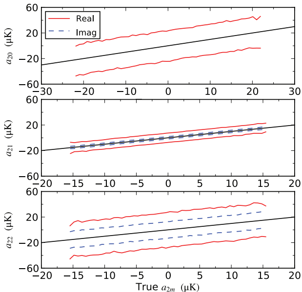
Figure 1. The 95th and 5th percentile lines for the a_{2m} reconstructed from the pixels outside the KQ75y7 mask at N_{\text{side}} = 128 (and thus \ell_{\text{max}} = 514 ) of \Lambda\text{CDM} realizations with C_2 = 100 (\mu\text{K})^2 , as discussed in the text. The red, solid lines are for the real part of the a_{2m} and the blue, dashed lines are for the imaginary part. The black, solid line shows the expected result for a perfect reconstruction. We see that the reconstruction is unbiased, that is it tracks the true value.
