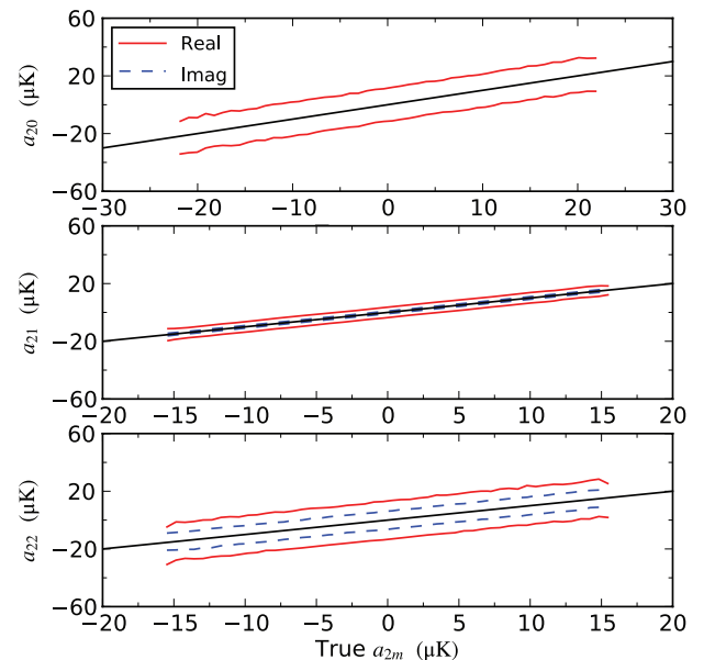
Figure 3. The same as Fig. 1, now reconstructed from maps smoothed with a 10^\circ Gaussian beam applied to the full-sky map. As in Fig. 1, the reconstruction is unbiased.
