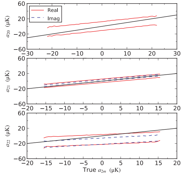
Figure 2. The same as Fig. 1, now reconstructed from the pixels outside the KQ75y7 mask at N_{\text{side}} = 16 (and thus \ell_{\text{max}} = 66 ). Here we see that the reconstruction is biased.
