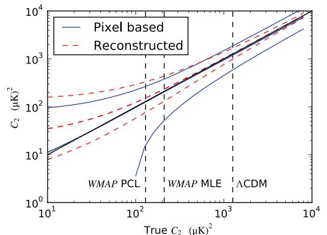
Figure 8. The same as Fig. 7, now with the realizations smoothed to 10^\circ prior to reconstruction. It appears that the estimator (16) does a better job of reproducing C_2 for a \Lambda CDM model, though see Fig. 9.
