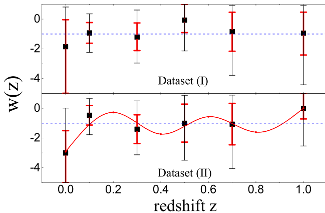
FIG. 1 (color online). Reconstruction of w(z) using the data sets I (top panel) and II (bottom panel); see text for details. The inner (red) and outer (black) error bars correspond to 68% and 95% error bars, respectively. The \Lambda CDM model is shown with the dashed (blue) line. In the bottom panel, we also plot the reconstruction result with an alternative placement of fitting nodes (points and curve; see text for details).
