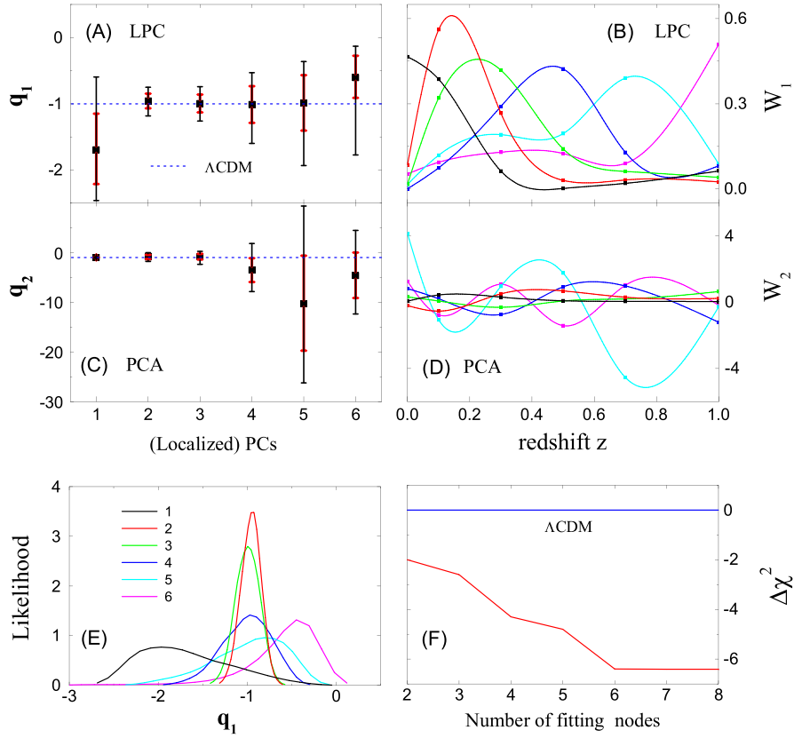
FIG. 2 (color online). Constraints on uncorrelated band powers of the equation of state w(z) , using the data set II. (a), (b) median values and the 68% and 95% constraints on the localized principal components \mathbf{q}_1 , and their weights in redshift \mathbf{W}_1 , respectively. (c), (d) same for the principal components \mathbf{q}_2 and their weights \mathbf{W}_2 (see the text for definitions). (e) likelihood distributions for the parameters \mathbf{q}_1 ; (f) reduction in \chi^2 relative to \Lambda CDM as the number of fitting nodes (for parameters \mathbf{q}_1 ) is increased.
