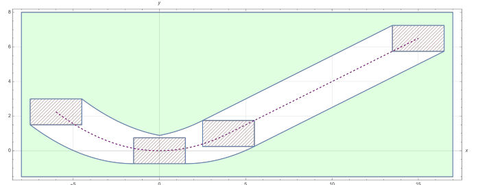
Fig. 9: Safe region for an instance of [21]. The notches are the red-hatched rectangles and the trajectory is dashed in purple.
