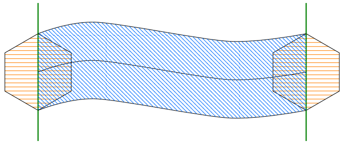
Fig. 5: Terms in Equation (6), illustrated. Green terms restrict test to relevant piecewise subdomains, blue, diagonally-hatched terms check if obstacles are between active corner pairs, and orange, horizontally-hatched terms check if obstacles are in the notch at transition points and subdomain bounds.
