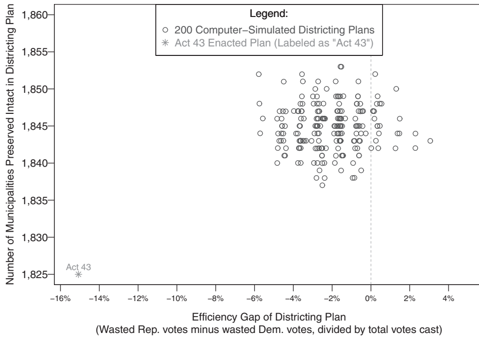
FIG. 3. Comparison of simulated districting plans to Act 43 on efficiency gap and preservation of municipal boundaries.
