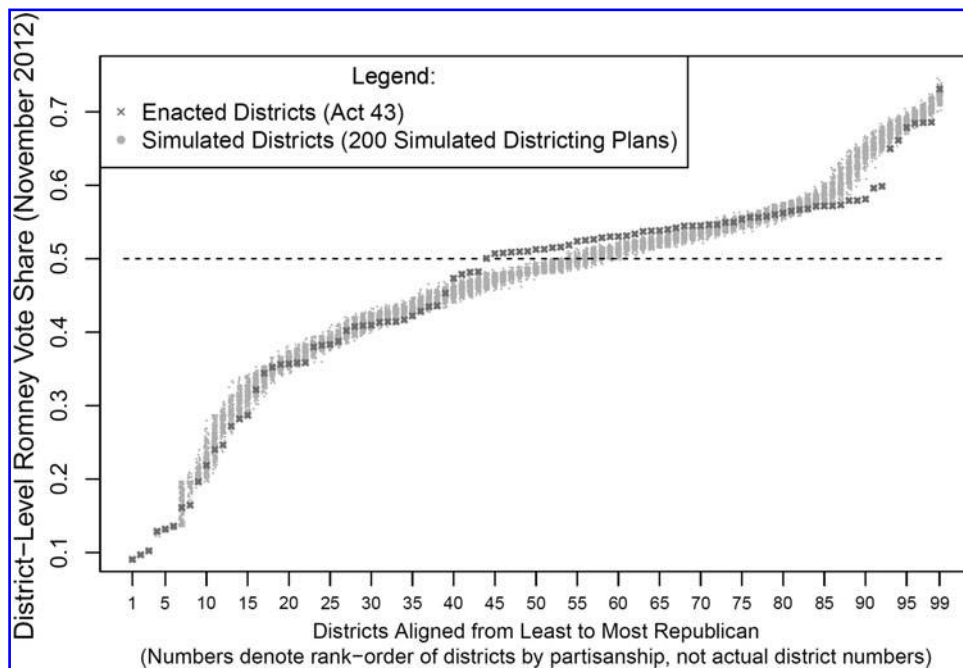
FIG. 7. Comparison of simulated vs. enacted (Act 43) districts.
