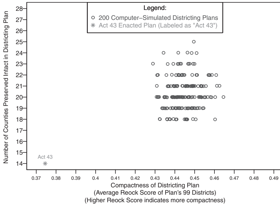
FIG. 1. Comparison of simulated districting plans to Act 43 on compactness and preservation of county boundaries.
