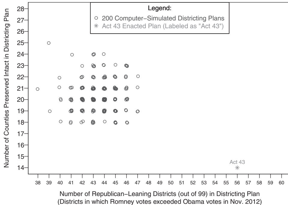
FIG. 5. Comparison of simulated districting plans to Act 43 on Republican seats and preservation of county boundaries.
