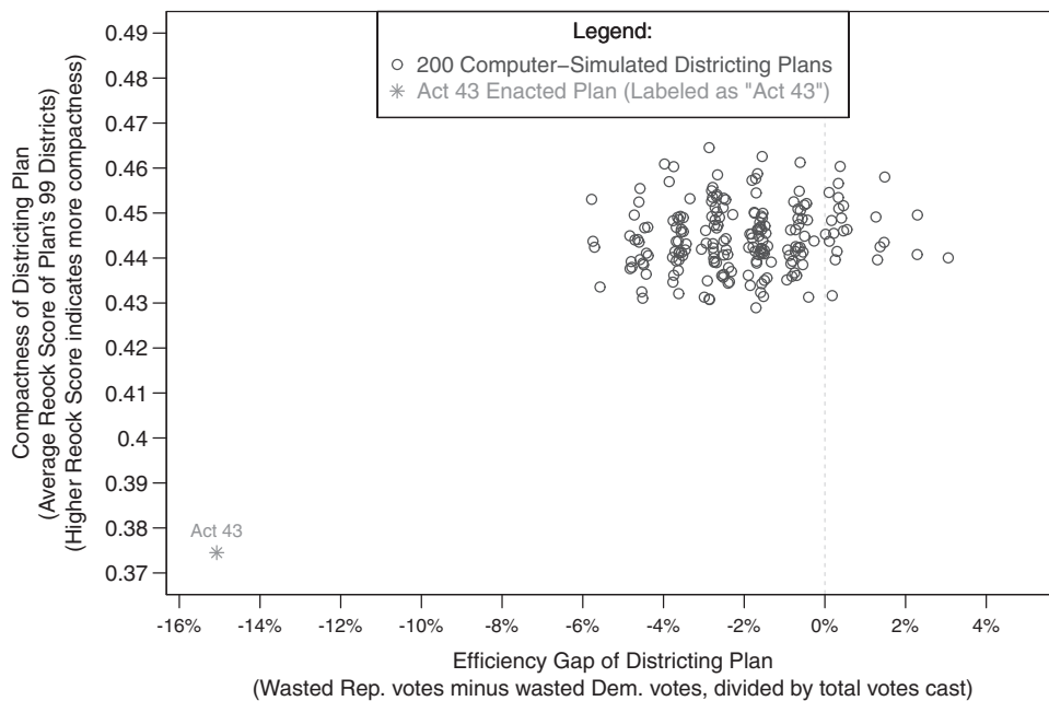
FIG. 4. Comparison of simulated districting plans to Act 43 on efficiency gap and compactness.
