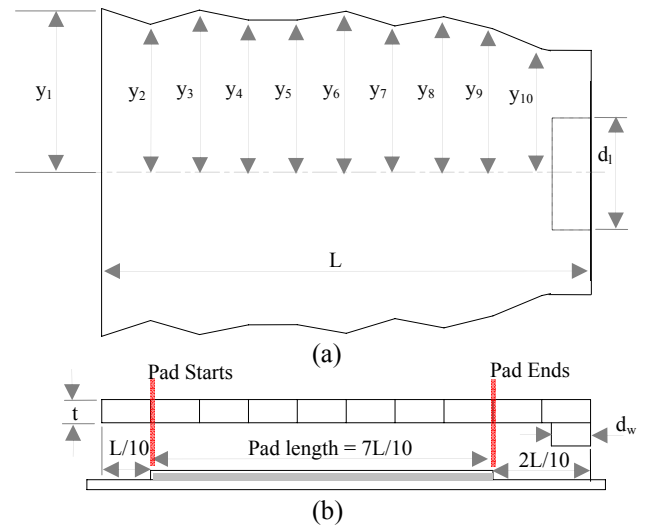
Figure 4: Switch geometry and design variables
