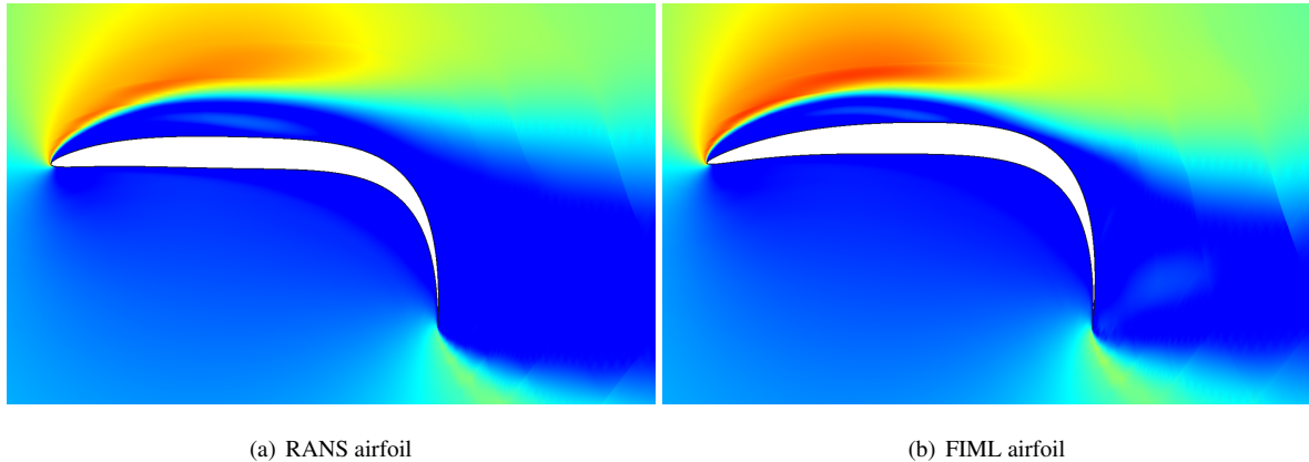
Figure 18: Time-averaged Mach number contours (0-.5) of airfoils optimized for lift maximization at M = 0.2, Re = 10^4 .
