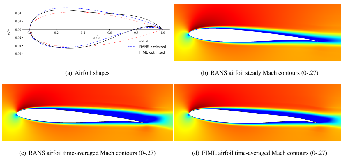
Figure 11: Comparison of RANS and FIML optimized airfoil shapes and time-averaged Mach number contours at M = 0.2, Re = 10^4, c_\ell = 0.4 .
