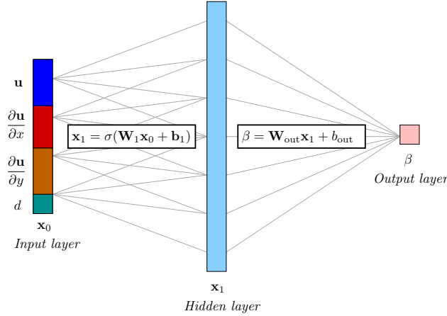
Figure 3: Structure of the artificial neural networks used to predict the correction field.
