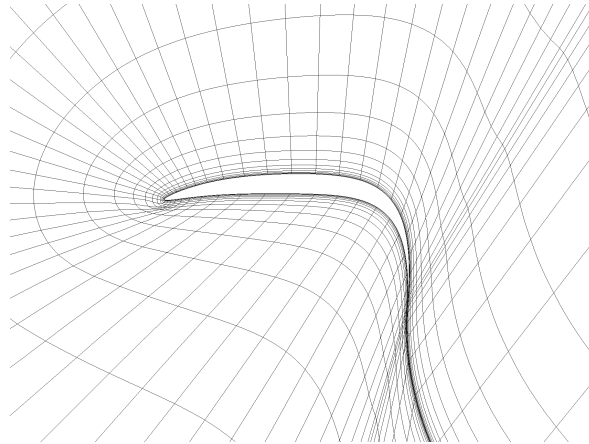
(c) Re = 10^4, \max(c_l) : 2112 elements
