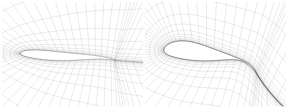
(a) Re = 10^4, c_l = 0.4 : 1978 elements
