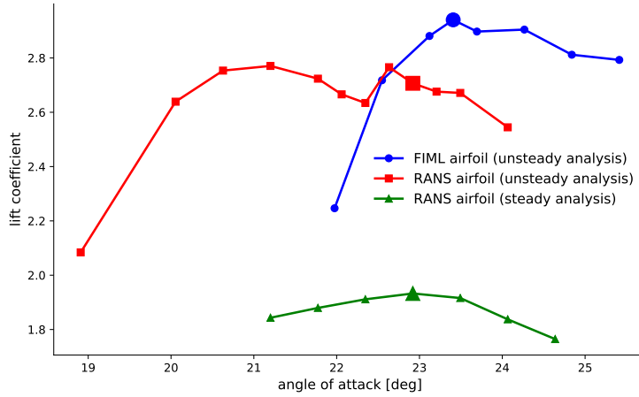
Figure 19: Lift coefficient versus angle of attack for the optimized airfoils for lift maximization at M = 0.2, Re = 10^4 . Large symbols indicate the angle of attack determined from the optimization.
