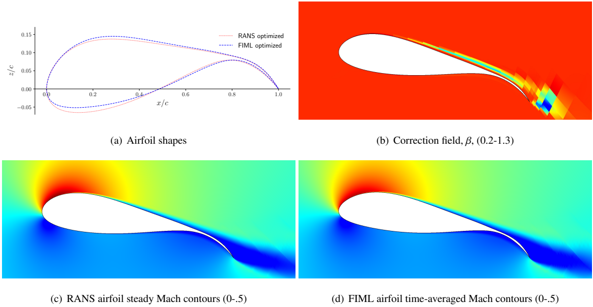
Figure 13: Comparison of RANS and FIML airfoil shapes, the correction field, and Mach number contours for drag minimization at M = 0.2 , Re = 10^6 , c_l = 2.4 .
