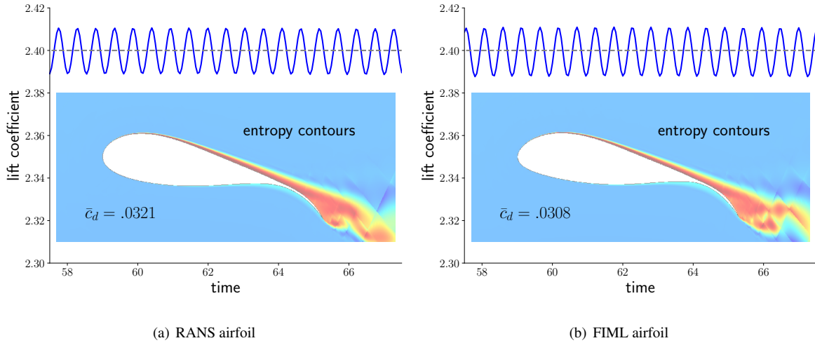
Figure 12: Unsteady analyses of RANS and FIML airfoils optimized for minimizing drag at M = 0.2 , Re = 10^6 , c_\ell = 2.4 .
