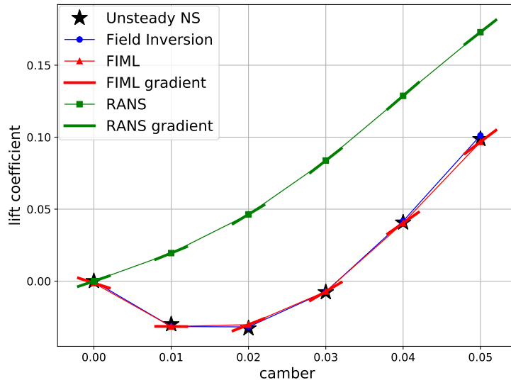
Figure 4: Field-inversion and machine learning results for lift-coefficient calculations in unsteady flow around NACA X412 airfoils at M = 0.2 , Re = 10^4 , \alpha = 0 .
