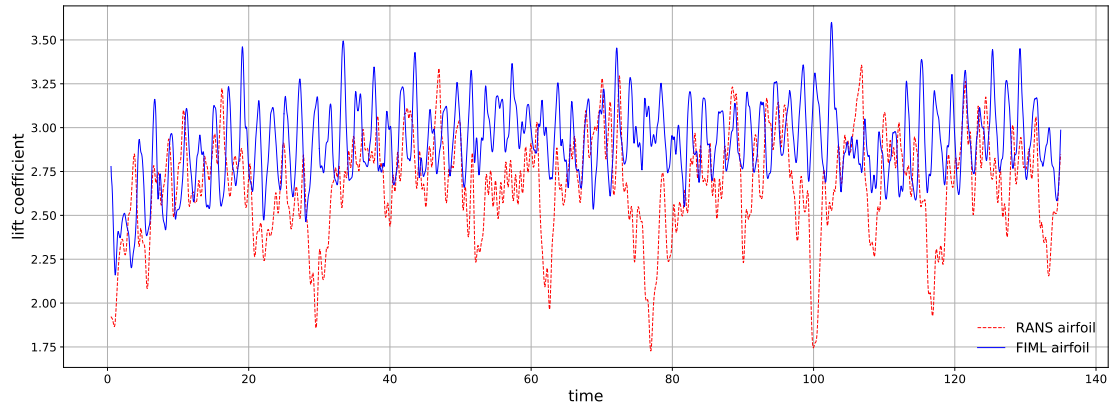
Figure 16: Lift coefficient time histories for lift maximization at M = 0.2, Re = 10^4 .
