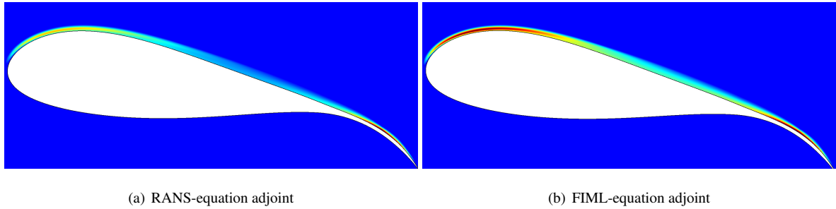
Figure 14: Field plots of the conservation of x -momentum component of the drag adjoint for the RANS-optimized airfoil, using both the RANS equations and the corrected, FIML equations at M = 0.2 , Re = 10^6 , c_l = 2.4 .
