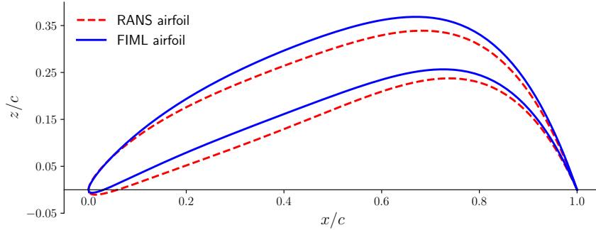
Figure 15: Airfoils optimized for maximum lift at M = 0.2, Re = 10^4 .
