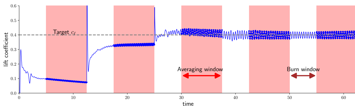
Figure 6: Unsteady trimming of the lift coefficient using the angle of attack, taken from a simulation of the airfoil studied in Section 7.1.
