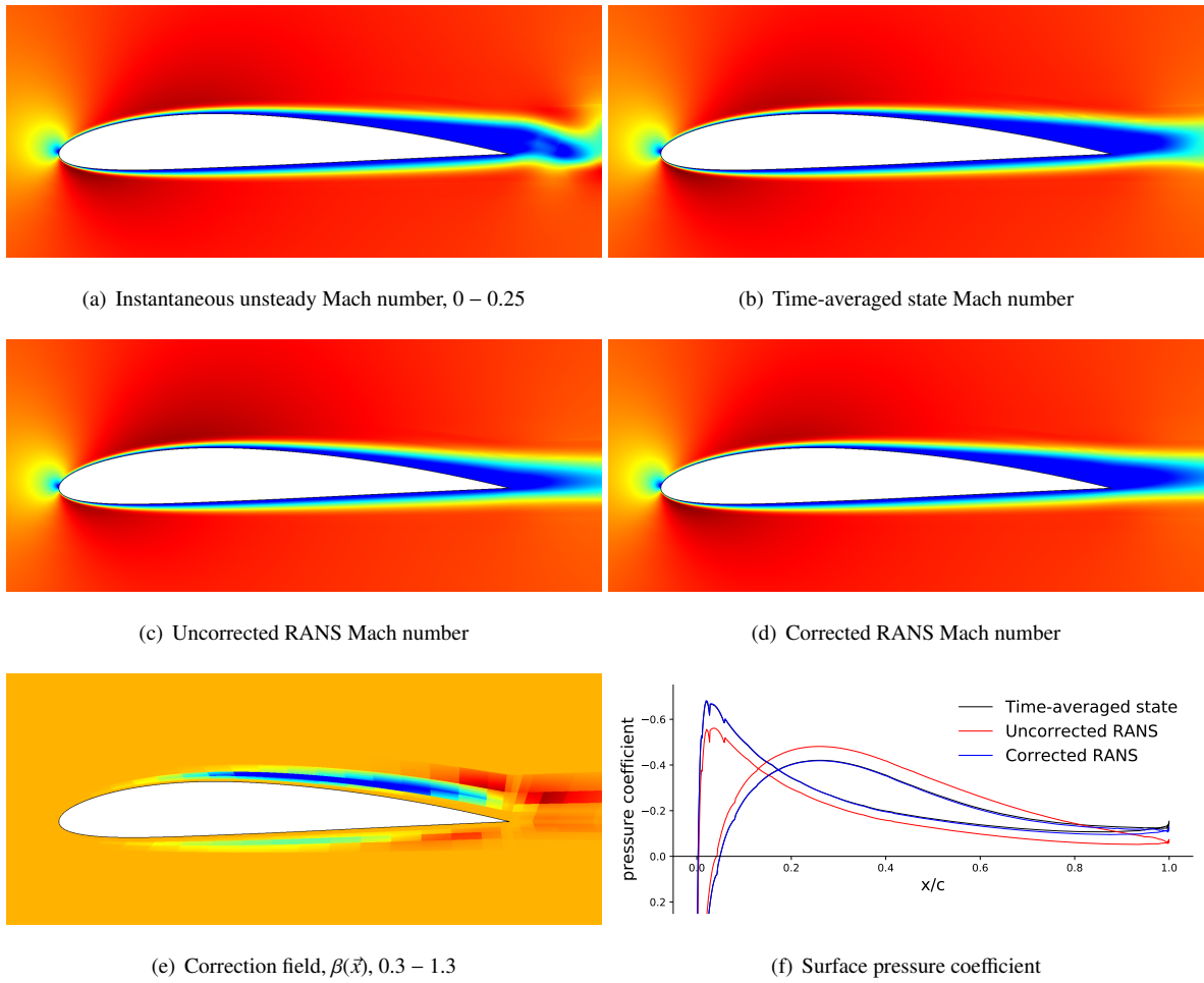
Figure 2: Field-inversion results for unsteady flow around a NACA 3412 airfoil at M = 0.2, Re = 10^4, \alpha = 0 .
