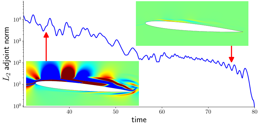
Figure 9: Instability in the unsteady lift-integral adjoint for the initial airfoil in the constrained-lift drag minimization at M = 0.2 , Re = 10^4 , c_\ell = 0.4 . Field plots show the conservation of x momentum adjoint. Time is measured in units of the airfoil chord divided by the freestream speed.
