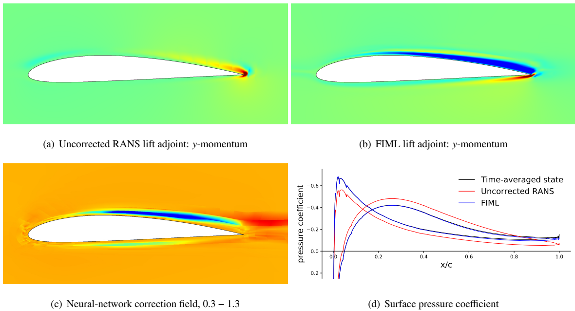
Figure 5: FIML and RANS contour plots for unsteady flow around a NACA 3412 airfoil at M = 0.2 , Re = 10^4 , \alpha = 0 .
