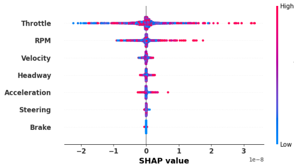
Fig. 3. SHAP summary
