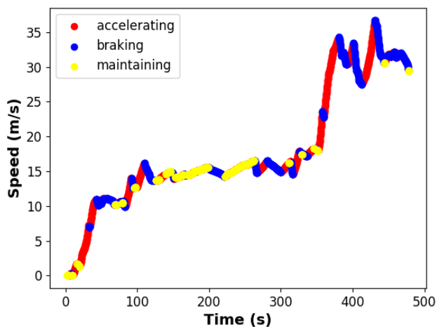
Fig. 1. Manoeuvre detection of a sample trip
