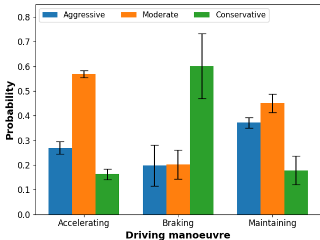
Fig. 2. Classification result of a sample driver
