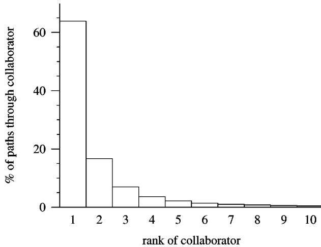
FIG. 2. The average percentage of paths from other scientists to a given scientist that pass through each collaborator of that scientist, ranked in decreasing order. The plot is for the Los Alamos Archive network, although similar results are found for other networks.
