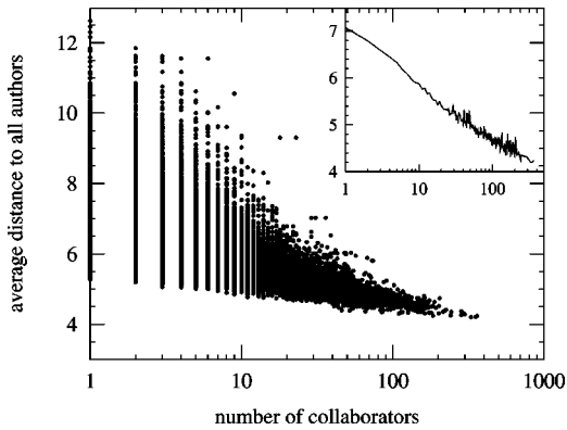
FIG. 5. Scatter plot of the mean distance from each physicist in the giant component of the Los Alamos Archive network to all others as a function of number of collaborators. Inset: the same data averaged vertically over all authors having the same number of collaborators.
