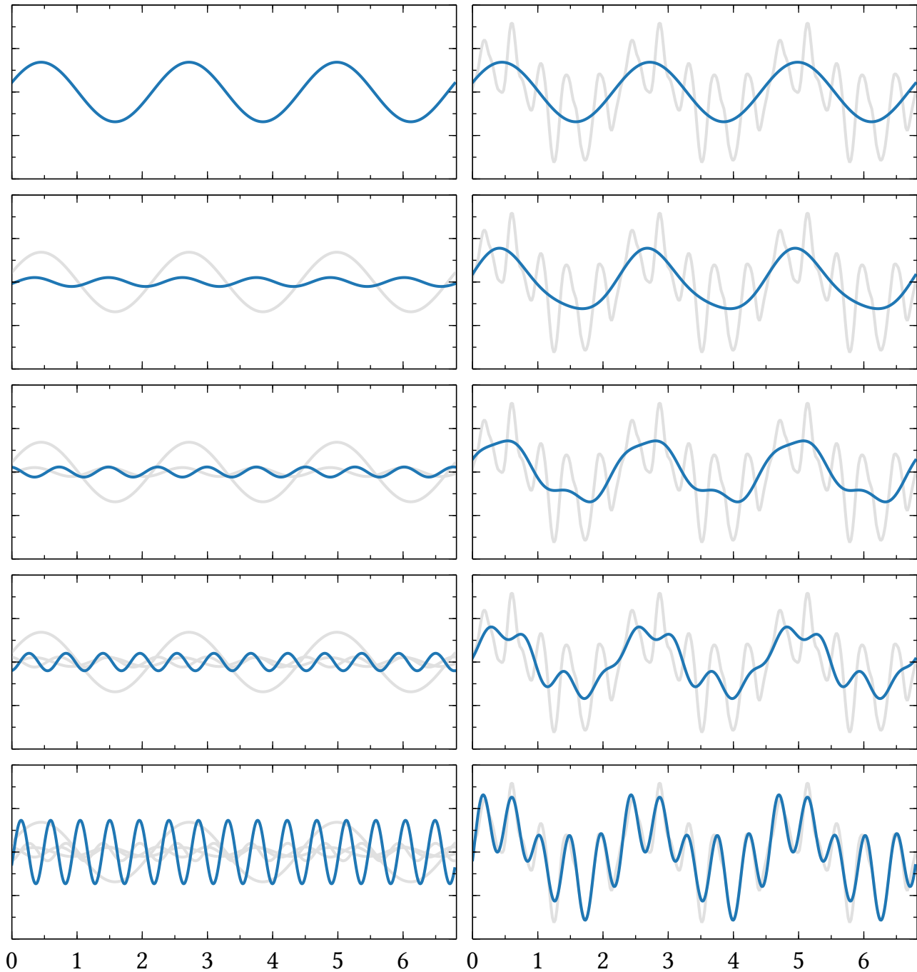
Resulting waveform
