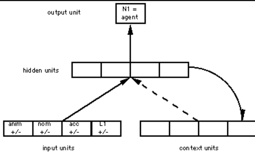
Figure 2b: Architecture of the recurrent neural network model
