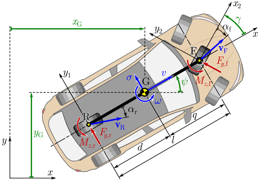
Figure 1. Traditional single track model which takes into account the lateral deformation of the tyres. The coordinate frames, the geometric and kinematic quantities, the lateral tyre forces and the aligning moments are shown in the figure.
