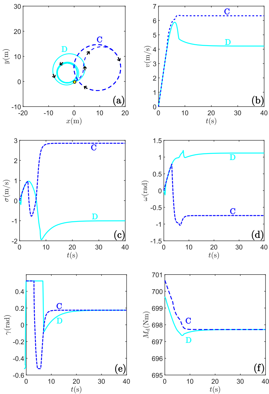
Figure 14. Simulation result for stabilising the drifting solution C and the donut solution D.
