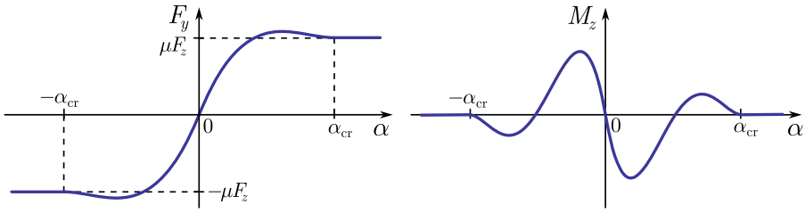
Figure 2. Lateral tyre force F_y and aligning torque M_z characteristics as the function of the tyre slip angle \alpha .
