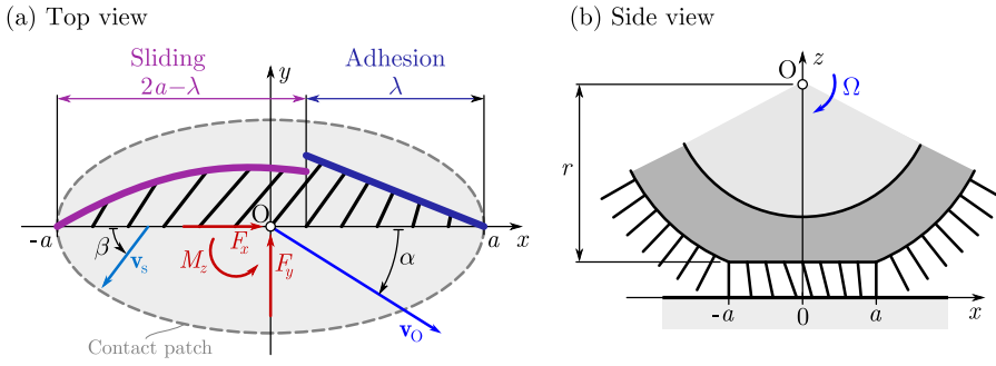
Figure 5. Combined slip brush tyre model highlighting the adhesion region and the sliding region and indicating the slip angle \alpha and the sliding angle \beta . The longitudinal and lateral tyre forces F_x and F_y , and the aligning moment M_z are also shown on the figure.
