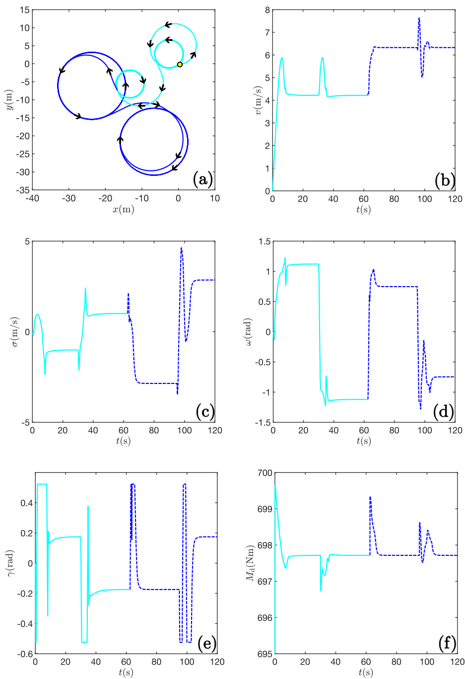
Figure 16. Simulation result when transitioning from donut figure eight manoeuvre to drifting figure eight manoeuvre by switching between four different controllers.
