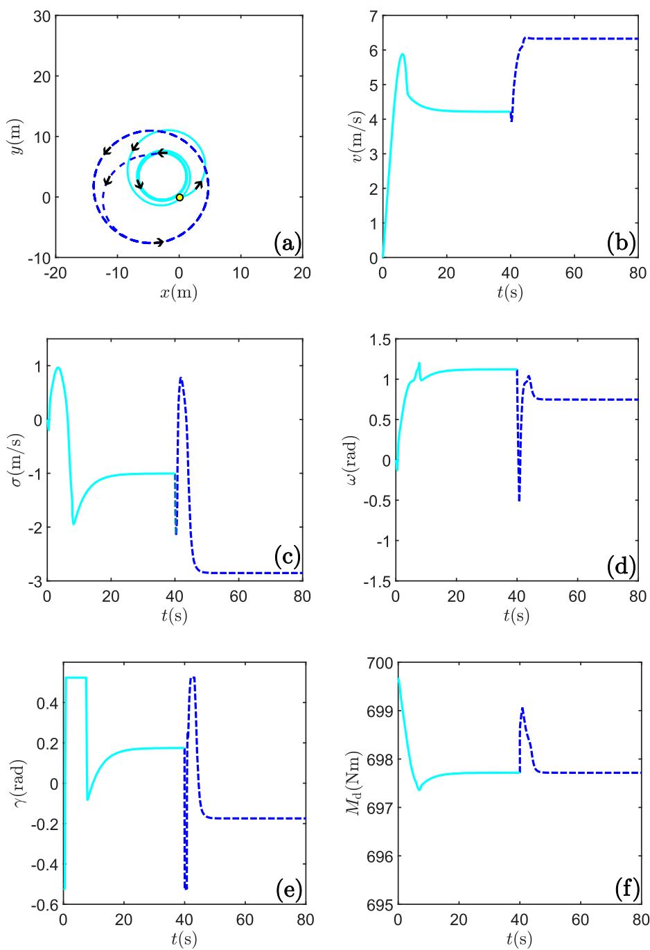
Figure 15. Simulation result when transitioning from donut to drifting by switching controllers.
