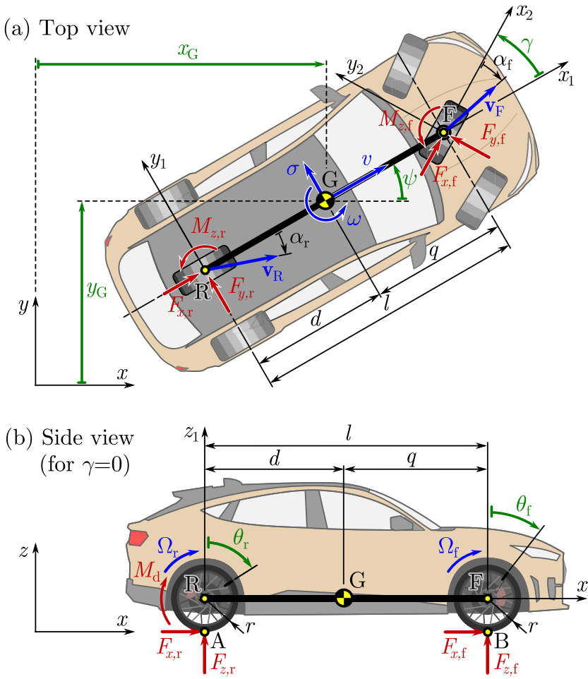
Figure 4. Higher fidelity single track model which takes into account both the lateral and the longitudinal deformation of the tyres. The coordinate frames, the geometric and kinematic quantities, the longitudinal and lateral tyre forces, and the aligning moments are shown in the figure.
