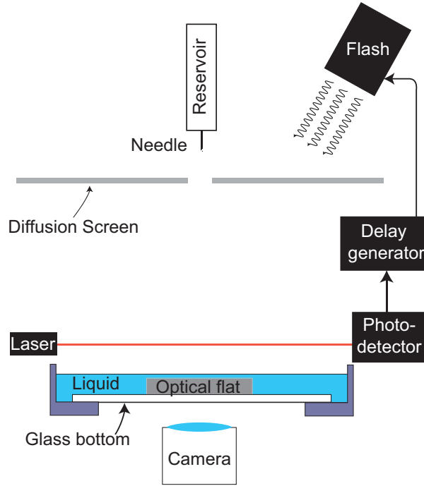
Figure 4. Experimental apparatus.
