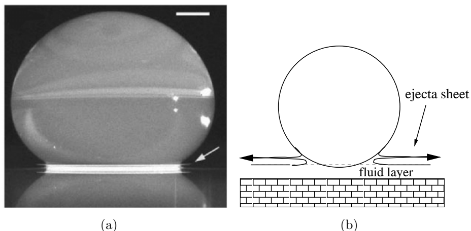
Figure 5. Left: An experimental snapshot of a drop directly after impact [15]. The parameters are Re = 1080 , We = 4170 . Right: A cartoon of the same process, following [17]. An ejecta sheet shoots out horizontally from underneath the drop.
