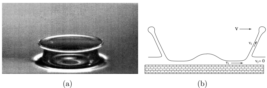
Figure 6. Left: an experiment corresponding to the cartoon on the right. The parameters are Re = 676 , We = 428 , 775 \mu s after impact. Corresponds to \bullet in Fig. 3. Right: A cartoon of the mechanism for sheet formation as proposed in [2]. Mass and momentum conservation determine the velocity and angle of the upward moving sheet, which usually rises at a steep angle.
