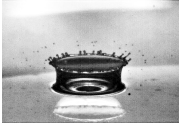
Figure 7. An ejecta sheet “riding” on a Peregrine sheet. The former leads to the formation of tiny droplets that precede the much larger Peregrine sheet. Re=1354 , We=874 , 580 \mu s after impact. Corresponds to ★ in Fig. 3.
