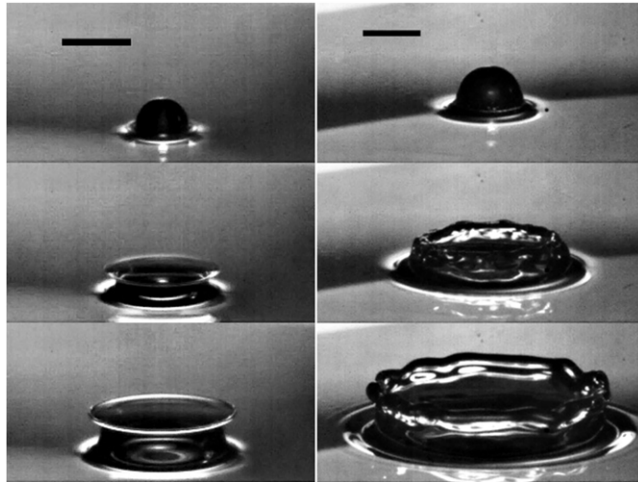
Figure 9. Smooth and disordered Peregrine sheets that do not produce secondary droplets. Left: silicon oil, Re = 676 , We = 428 , H = 0.2 at 100, 368, 775 \mu s after impact. Corresponds to circle in figure 3. Right: water, Re = 4226 , We = 106 , H = 0.2 at 300, 1650, 4215 \mu s after impact. Corresponds to \blacklozenge in figure 3. Scale bar corresponds to 2 mm.
