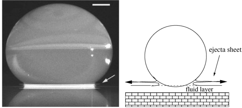
Figure 5. Left: an experimental snapshot of a drop directly after impact [15] (reproduced courtesy of Cambridge University Press). The parameters are Re = 1080 , We = 4170 . Right: a diagram of the same process, following [17]. An ejecta sheet shoots out horizontally from underneath the drop.
