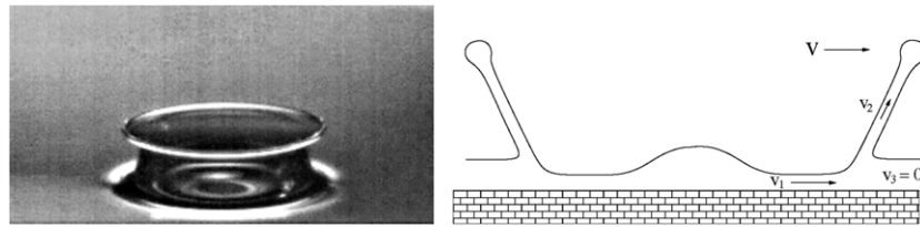
Figure 6. Left: an experiment corresponding to the diagram on the right. The parameters are Re = 676 , We = 428 , 775 \mu s after impact. Corresponds to ● in figure 3. Right: a diagram of the mechanism for sheet formation as proposed in [2]. Mass and momentum conservation determine the velocity and angle of the upward moving sheet, which usually rises at a steep angle.
