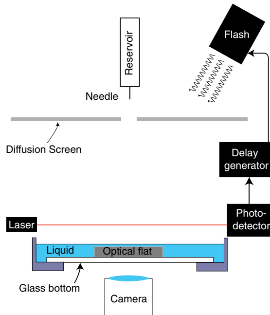
Figure 4. Experimental apparatus.
