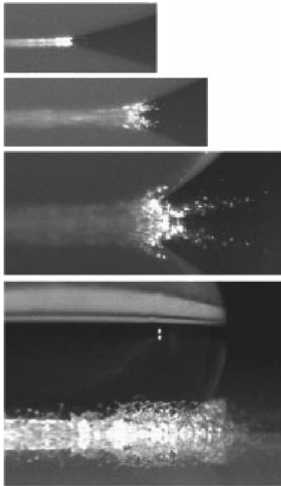
Figure 8. An ejecta sheet breaking up into many smaller droplets, at a stage where the sheet is still hidden completely underneath the drop [15] (reproduced courtesy of Cambridge University Press). The parameters are Re = 2.9 \times 10^4 and We = 1.8 \times 10^3 .
