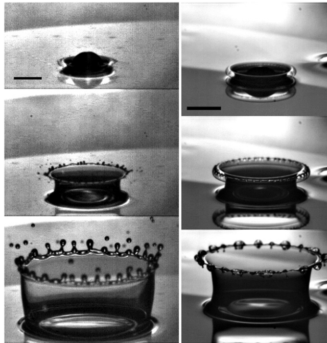
Figure 11. Left: drop impact producing both a microdroplet and crown splash. Propanol, Re = 1816 , We = 582 , H = 0.2 at 160, 570, 2650 \mu s after impact. Corresponds to \star in figure 3. Right: splash which entrains bubbles in to the Peregrine sheet rim. Silicon oil, Re = 1392 , We = 1326 , H = 0.2 at 200, 610, 1010 \mu s after impact. Corresponds to \blacksquare in figure 3. The scale bar corresponds to 2 mm.
