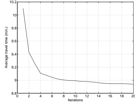
Fig. 4. The evolution of best values as a function of iteration count for the light-flow case.
