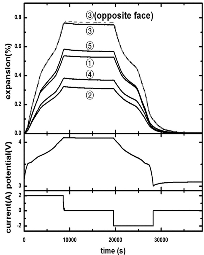
Fig. 2. Expansion (swelling) trends over time; encircled digits indicate measurement points shown in Fig. 1; the measured current and potential over time are shown in the bottom plots.
