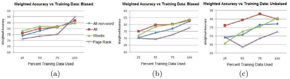
Fig. 1. Variation of weighted accuracy with percent training data used in the (a) heavily biased ( \lambda = 3 ), (b) moderately biased ( \lambda = 2 ), and (c) unbiased ( \lambda = 1 ) cases
