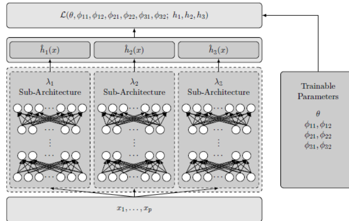
Figure 10 Architecture for the proposed semi-competing risk deep neural network.
